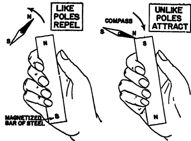
Law of magnetism.
